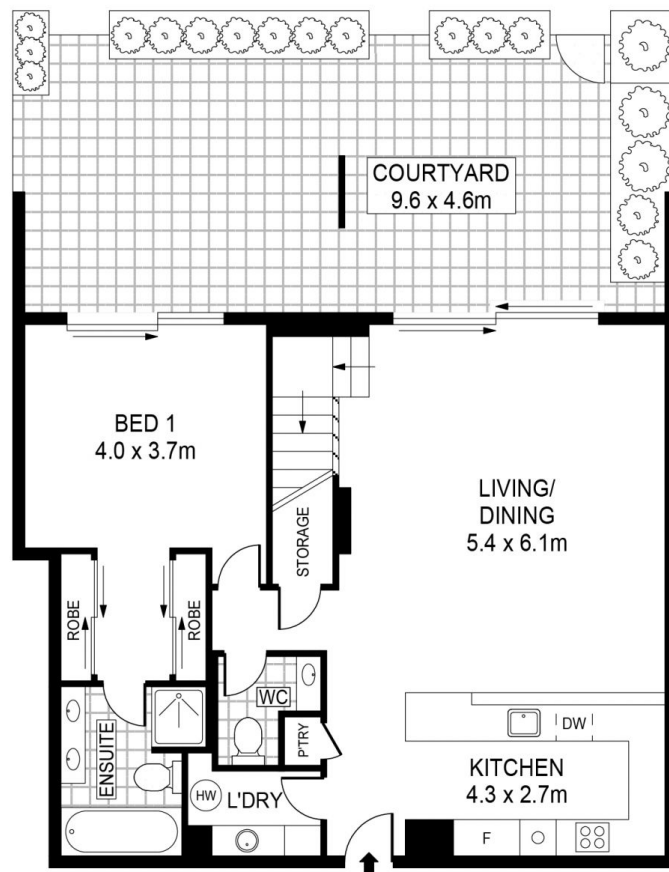
LEVEL ONE
